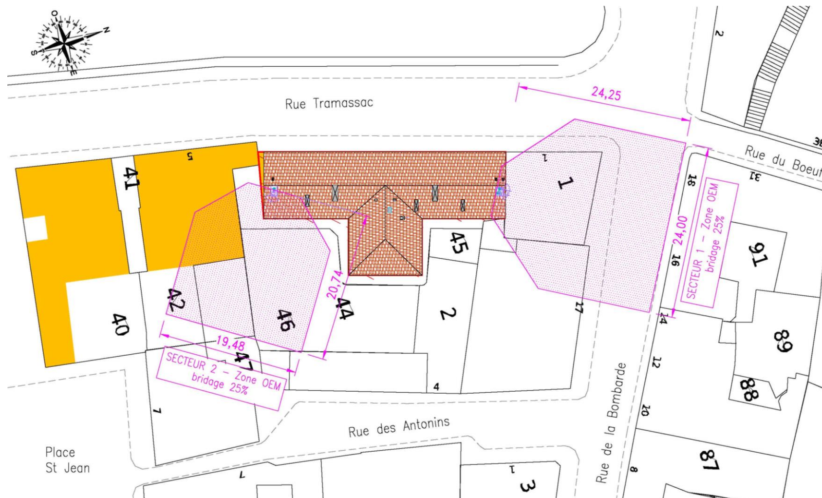
PERIMETRE DE SECURITE BOUYGUES TELECOM
